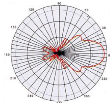
Vertical Pattern
